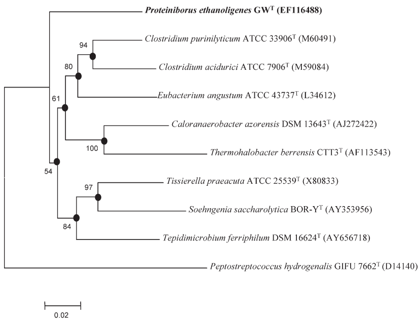
Fig. 1. Phylogenetic dendrogram of 16S rRNA gene sequences indicating the position of strain GW T among the bacterial members in cluster XII of the 'Clostridia'. The tree rooted with Peptostreptococcus hydrogenalis was constructed using the neighbour-joining method. Solid circles indicate that the corresponding nodes (groups) are also recovered in UPGMA and minimum evolution methods. Numbers at nodes represent levels of bootstrap support (%) based on a neighbour-joining analysis of 1000 resampled datasets. GenBank accession numbers of 16S rRNA sequences are given in parentheses. Bar, 2% sequence divergence.
