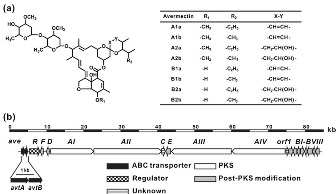
Fig. 1 Avermectins and S. avermitilis avermectin biosynthetic gene cluster. a Structures of eight avermectins. Avermectin B1a is the medically most effective compound. b S. avermitilis 80-kb avermectin ( ave ) biosynthetic gene cluster, and the avtAB operon encoding a
